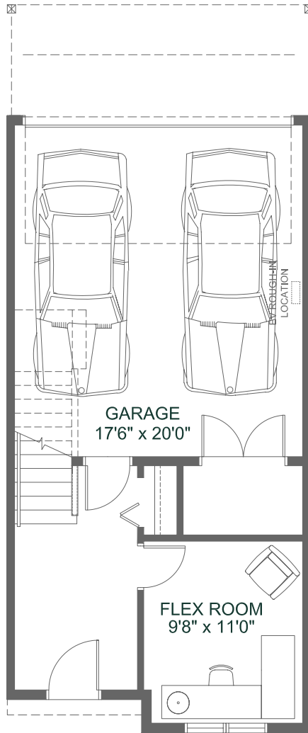
Ground Floor 234 SQ FT
