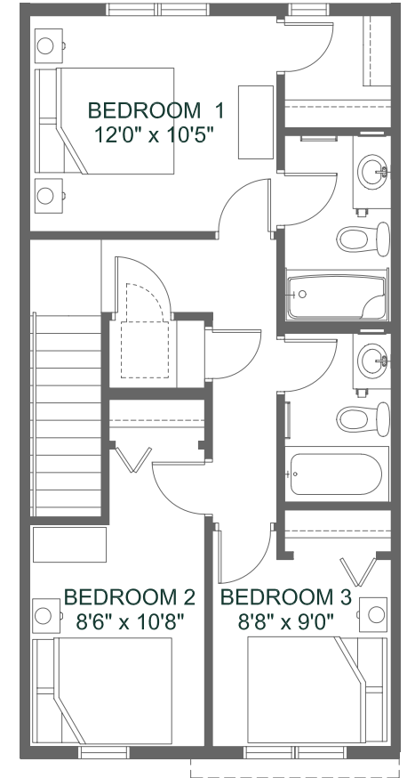
Third Floor 654 SQ FT
