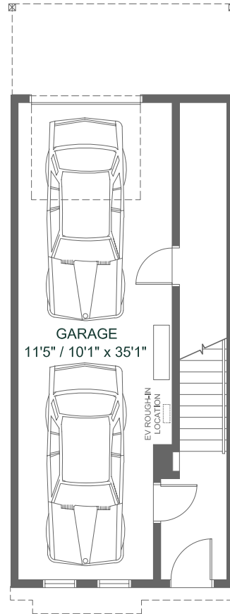
Ground Floor 57 SQ FT
