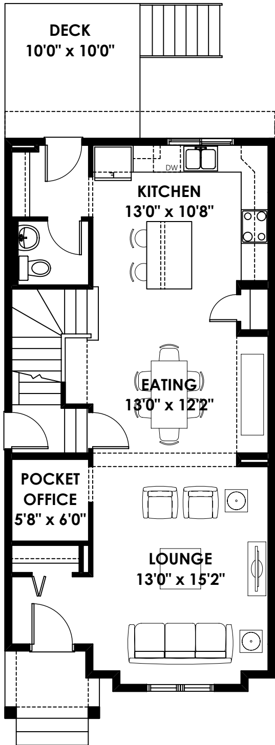
MAIN 798 SQ FT
