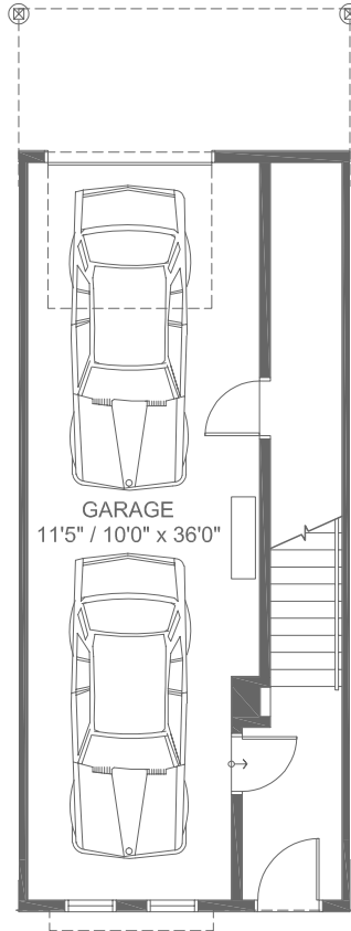
Ground Floor 63 SQ FT
