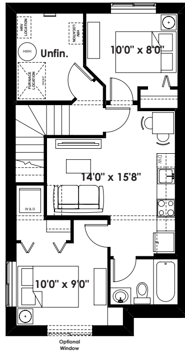
Optional 2 Bedroom Basement Suite Layout 523 Sq. Ft. (Finished Area; Must Add Optional Side Entry; Must Add 9' Foundation Walls)
