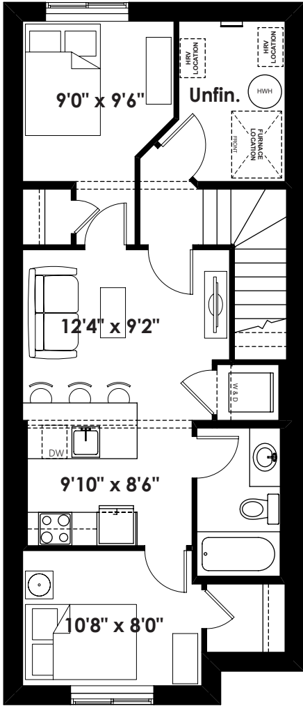
Optional 2 Bedroom Basement Suite Layout 554 Sq. Ft. (Finished)
