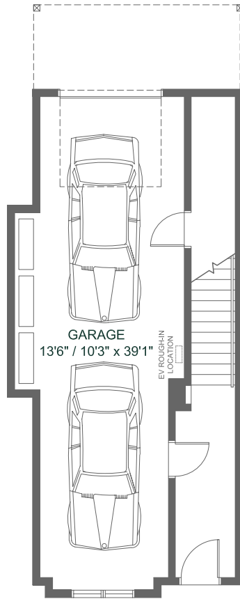
Ground Floor 88 SQ FT
