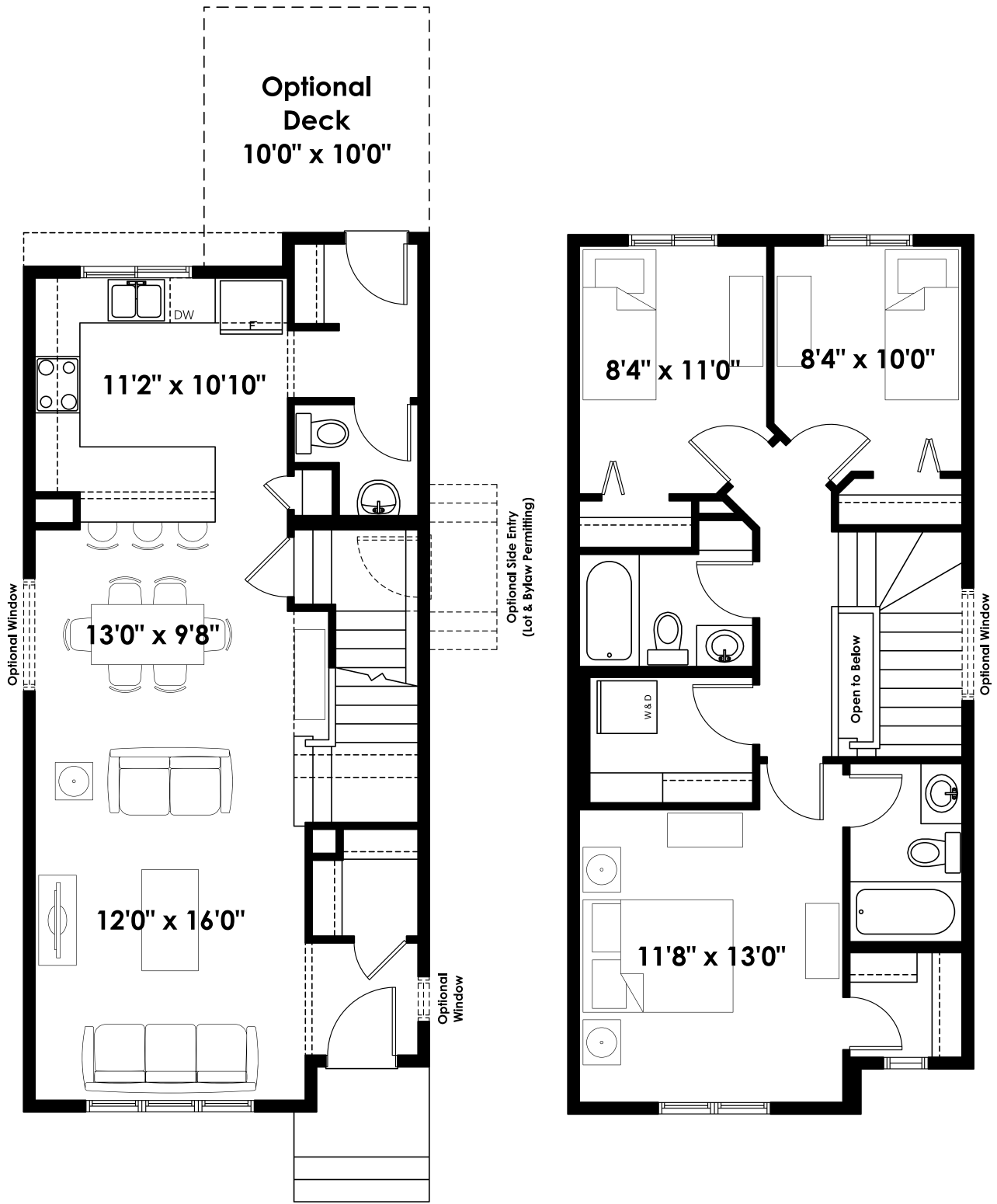
MAIN 675 SQ FT
