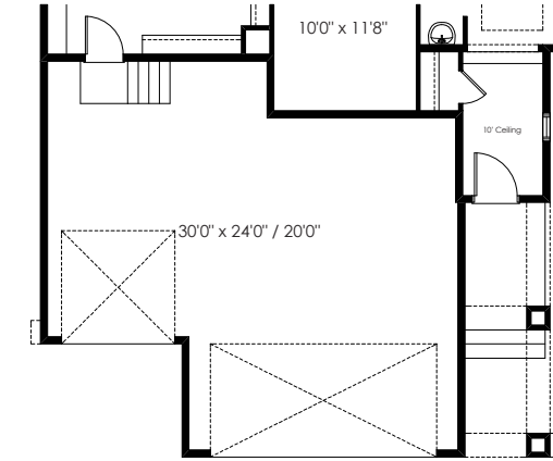
Partial Main Floor Plan for Macintosh - AC-1 Elevation (Adds 0 Sq. Ft. to main Floor)
