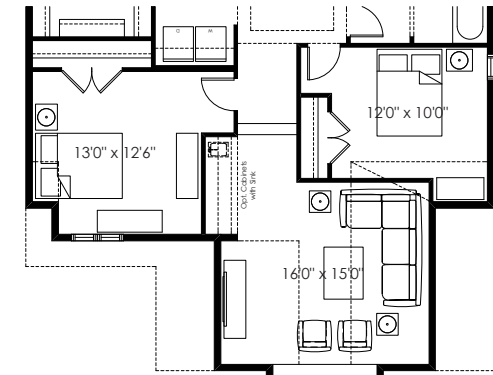
Partial Second Floor Plan for Macintosh - AC-1 Elevation (Adds 14 Sq. Ft. to Second Floor)
