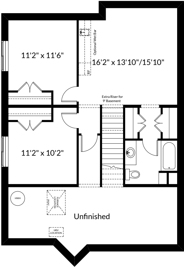
Alternate Two Bedroom Future Basement Room Layout 747 Sq. Ft. (Finished Area; Not Included in Contract)
