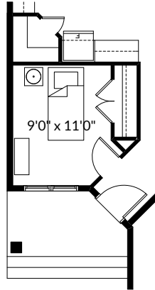
Partial Sedona Main Floor Plan with Optional Second Bedroom (Adds 0 Sq. Ft.)
