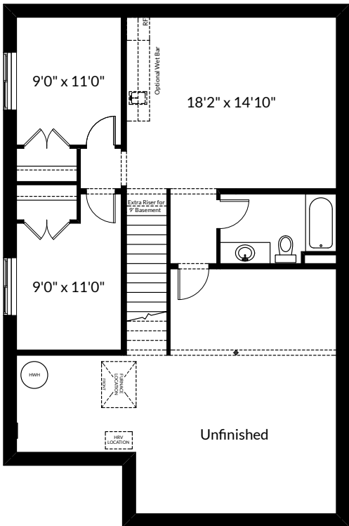
Alternate Two Bedroom Future Basement Room Layout 698 Sq. Ft. (Finished Area; Not Included in Contract)
