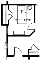
Partial Main Floor Plan with Optional Main Floor Bedroom (Adds 16 Sq. Ft. to Main Floor)
