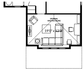
Partial Second Floor Plan for Wellesley - G1 & K1 Elevations (Removes 2 Sq. Ft. from Second Floor)
