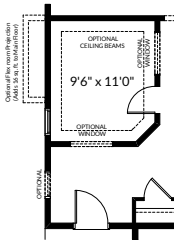
Partial Main Floor Plan with Optional Main Floor Office (Adds 0 Sq. Ft. to Main Floor)
