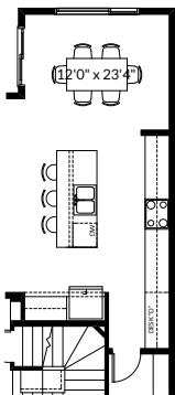
Partial Main Floor Plan with Optional Alternate Kitchen (Adds 26 Sq. Ft. to Main Floor)
