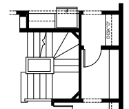
Partial Main Floor Plan with Optional Finished Stair to Basement with Opening (Adds 0 Sq. Ft. to Main Floor; Must Add 52 Sq. Ft. of Finished Basement Area Minimum)
