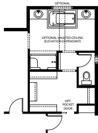
Partial Second Floor Plan with Optional Ensuite with 5' Shower (Adds 52 Sq. Ft. to Second Floor; Not Available on Optional Second Floor with Ensuite for Bedroom 3 & Optional 4 Bedroom Second Floors)
