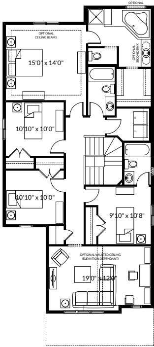
Optional 4 Bedroom Second Floor Plan with Ensuite for Bedroom 4 for Wellesley - Base Elevation (Adds 115 Sq. Ft. to Second Floor)
