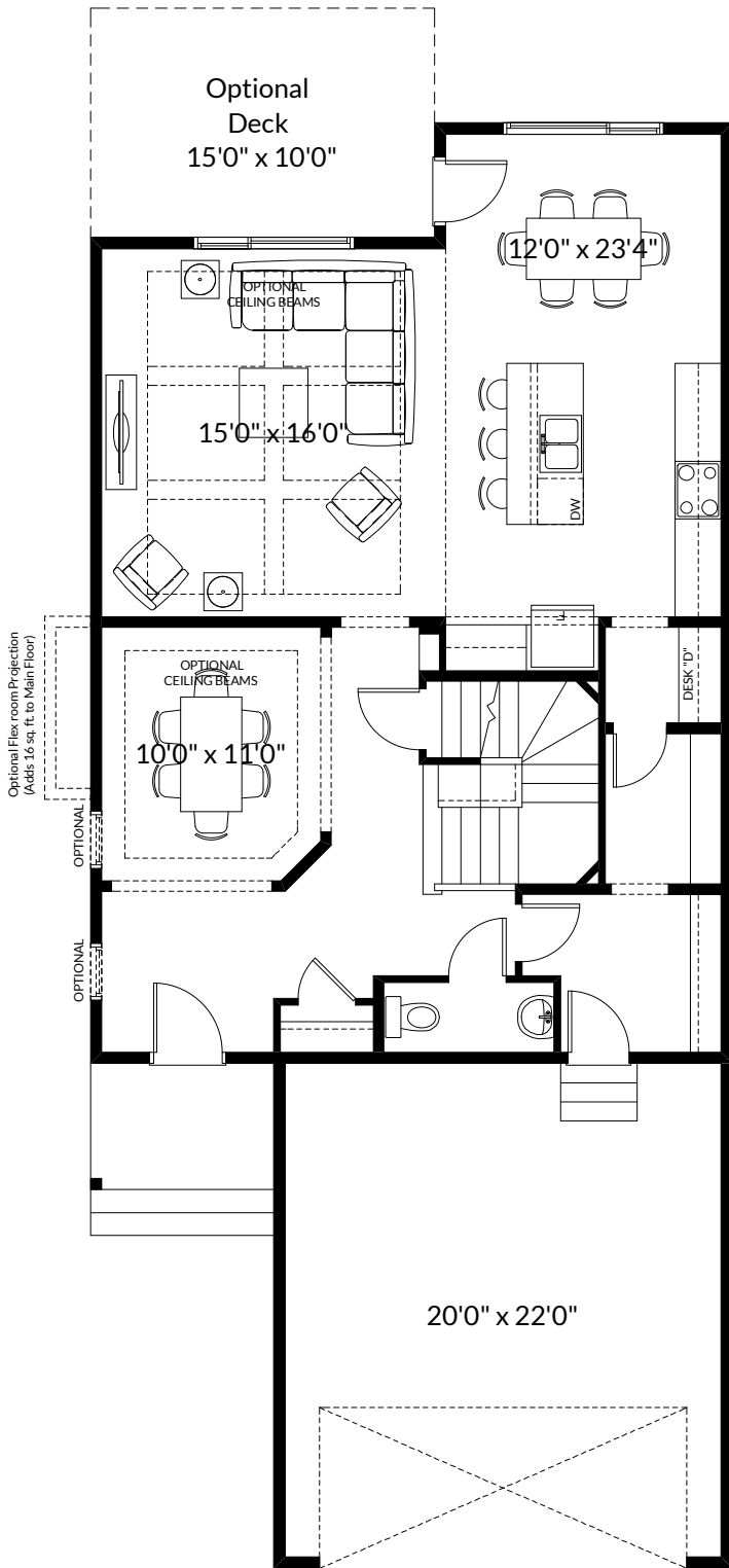
MAIN 1,073 SQ FT
