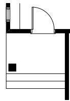
Partial Main Floor Plan for Rosedale - C3 & N1 Elevations (Adds 0 Sq. Ft. to Main Floor)
