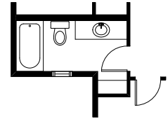
Partial Second Floor Plan with Optional Main Bath Vanity Extension (Adds 0 Sq. Ft. to Second Floor)
