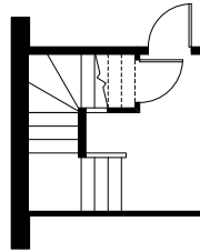
Basement Landing for Optional Finished Stair to Basement with Opening Adds 60 Sq. Ft. (Finished Area)
