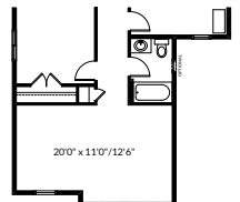
Partial Second Floor Plan for Caldwell - Q2 & Q3 Elevations (Adds 7 Sq. Ft. to Second Floor)
