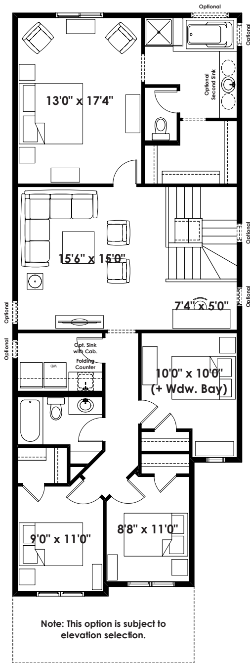
Second Floor Plan with Optional 4 Bedroom Layout (Adds 53 Sq. Ft. to Second Floor)
