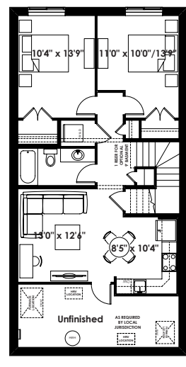
Optional Two Bedroom Basement Suite Layout 790 Sq. Ft. (Finished Area; Must Add Optional Side Entry)
