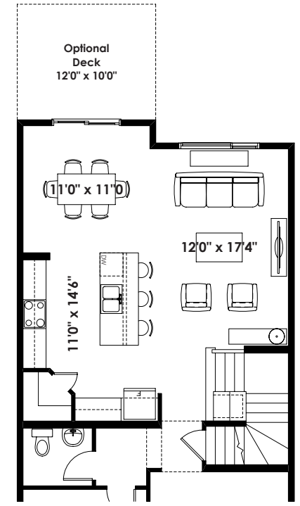
Partial Main Floor Plan with Optional Eating Area Extension (Adds 24 Sq. Ft. to Main Floor)
