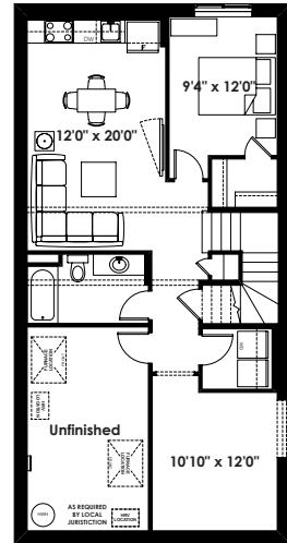
Optional Basement Suite Layout 780 Sq. Ft. (Finished Area)
