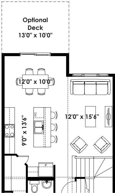
Partial Main Floor Plan with Optional Extended Kitchen (Adds 26 Sq. Ft. to Main Floor)
