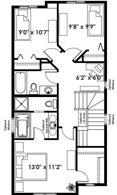
HARRELSON (Laundry Moves to Basement) Second Floor Plan (Adds 0 Sq. Ft. to Second Floor)
