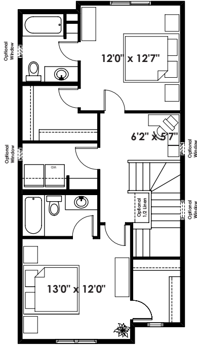
HOWE Second Floor Plan (Adds 0 Sq. Ft. to Second Floor)
