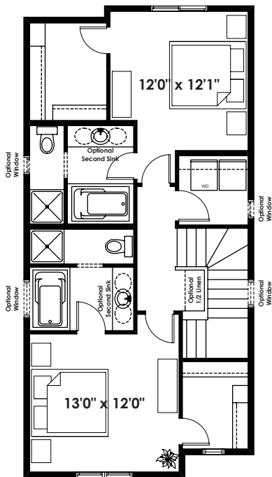
NORMAN Second Floor Plan (Adds 0 Sq. Ft. to Second Floor)
