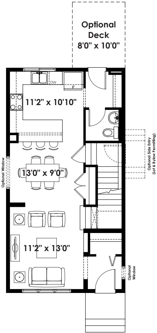
STELLAN Main Floor Plan With Optional Kitchen Layout (Adds 0 Sq. Ft. to Main Floor)
