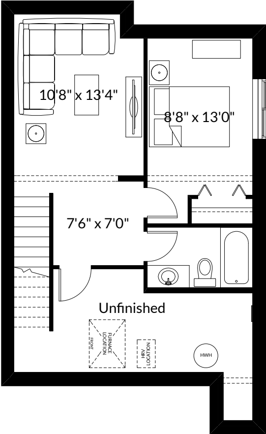
Optional Basement Room Layout 424 Sq. Ft. (Finished Area)
