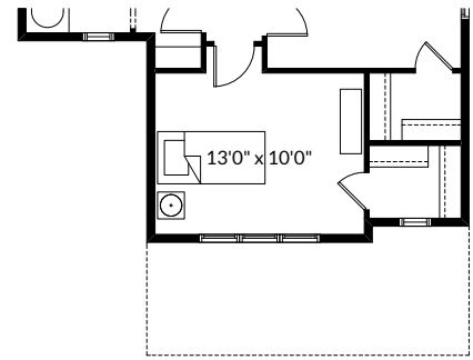
Partial Second Floor Plan for Rosedale - C3, J1, J2 & N1 Elevations (Adds 0 Sq. Ft. to Second Floor)
