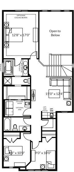
Second Floor Plan with 3 Bedrooms, Loft with Bar and Second Floor Laundry Room for Hawthorne - Base Elevation (Adds 0 Sq. Ft. to Second Floor) Note: This option is subject to elevation selection.
