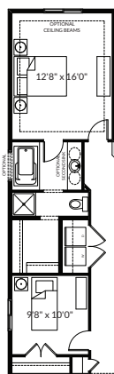
Partial Second Floor Plan with Optional Laundry Closet (Adds 0 Sq. Ft. to Second Floor)
