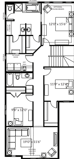
Second Floor Plan with 3 Bedrooms, Upgraded Ensuite and Second Floor Laundry Room for Hawthorne - Base Elevation (Adds 200 Sq. Ft. to Second Floor Must be combined with Optional Kitchen/Nook Extension)
