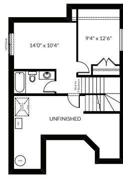
Optional Basement Room Layout for Optional Extended Garage 416 Sq. Ft. (Finished)
