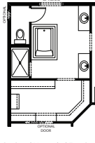
Optional Upgraded Ensuite #2 For Use with Second Floor Plan with 3 Bedrooms and Second Floor Laundry (Adds 200 Sq. Ft. to Second Floor Must be combined with Optional Kitchen/Nook Extension)
