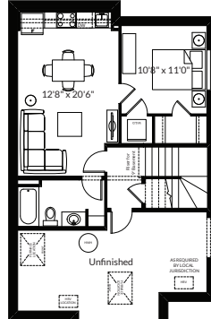
Optional Basement Suite Layout for Optional Nook Extension 573 Sq. Ft. (Finished Area; Must Add Optional Side Entry)
