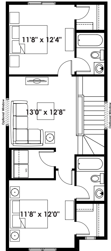
HENRY Second Floor Plan 777 Sq. Ft. Double Master Suite Upper Floor
