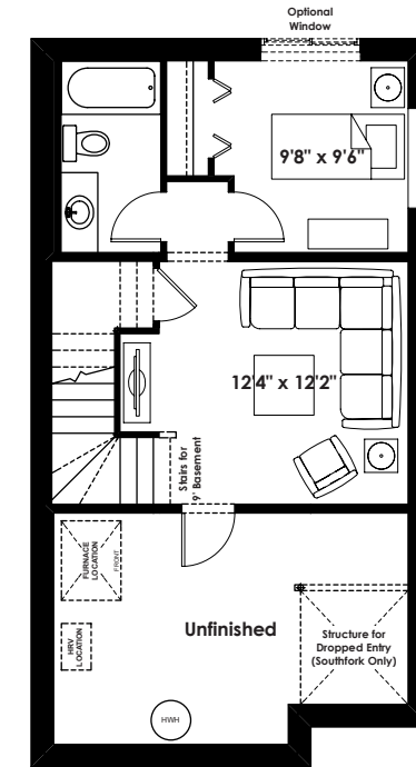
ALEXANDER Alternate Optional Basement Room Layout 374 Sq. Ft. (Finished)
