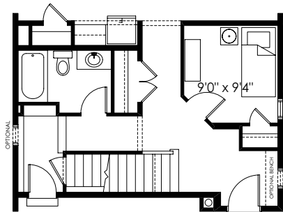
Partial Main Floor Plan with Optional Bedroom & 3 Piece Bathroom (Adds 0 Sq. Ft. to Main Floor)
