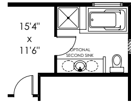
Partial Second Floor Plan with Optional Upgraded Ensuite #1 (Adds 0 Sq. Ft. to Second Floor)
