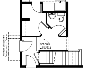
Partial Main Floor Plan with Optional Side Entry Door at Garage Landing (Adds 0 Sq. Ft. to Main Floor; Lot & Bylaw Permitting) NOTE: BASEMENT STAIR UNFINISHED
