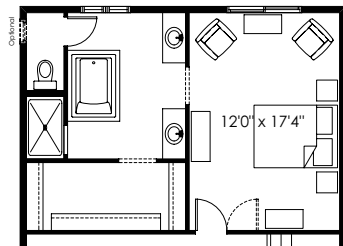
Partial Second Floor Plan with Optional Alternate Ensuite Layout (Adds 0 Sq. Ft. to Second Floor)
