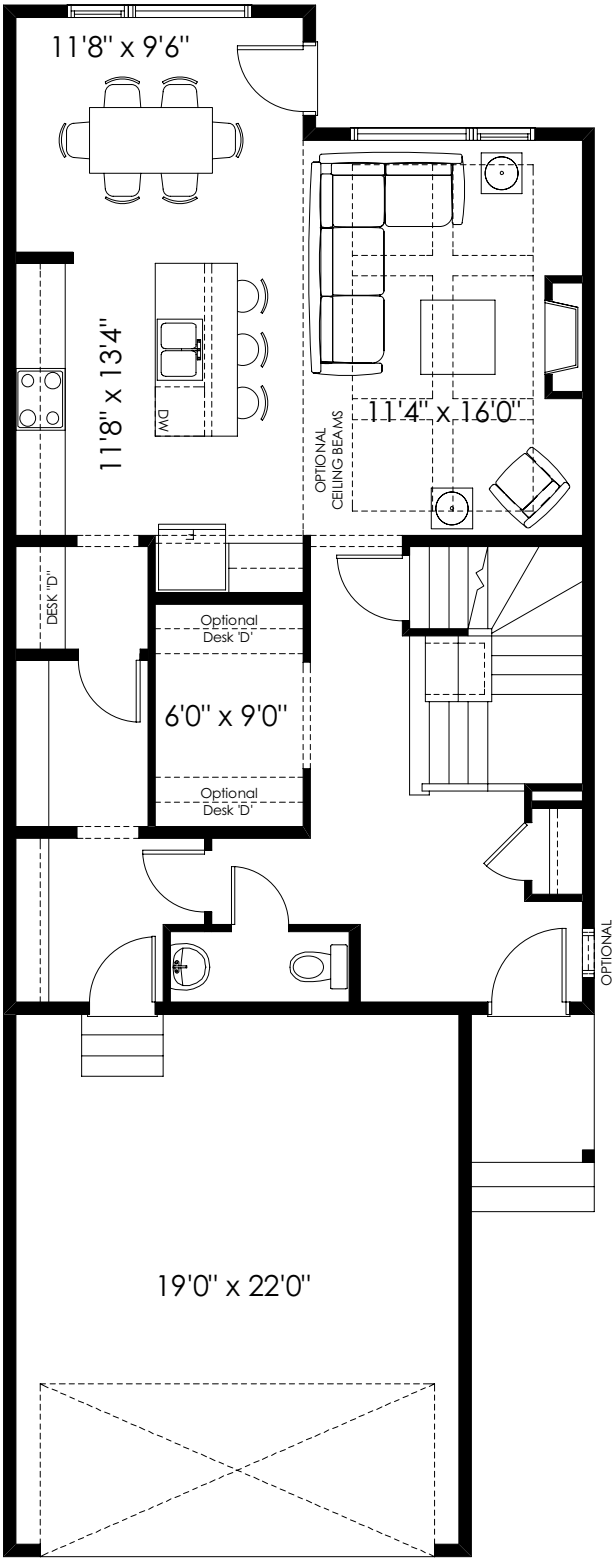
Main Floor 927 SQ FT
