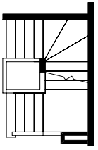
Partial Main Floor Plan with Optional Finished Stair to Basement with Opening (Adds 0 Sq. Ft. to Main Floor; Must Add 56 Sq. Ft. of Finished Basement Area Minimum)
