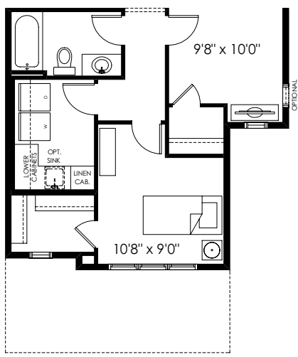
Partial Second Floor Plan with Optional Laundry Layout (Adds 0 Sq. Ft. to Second Floor)
